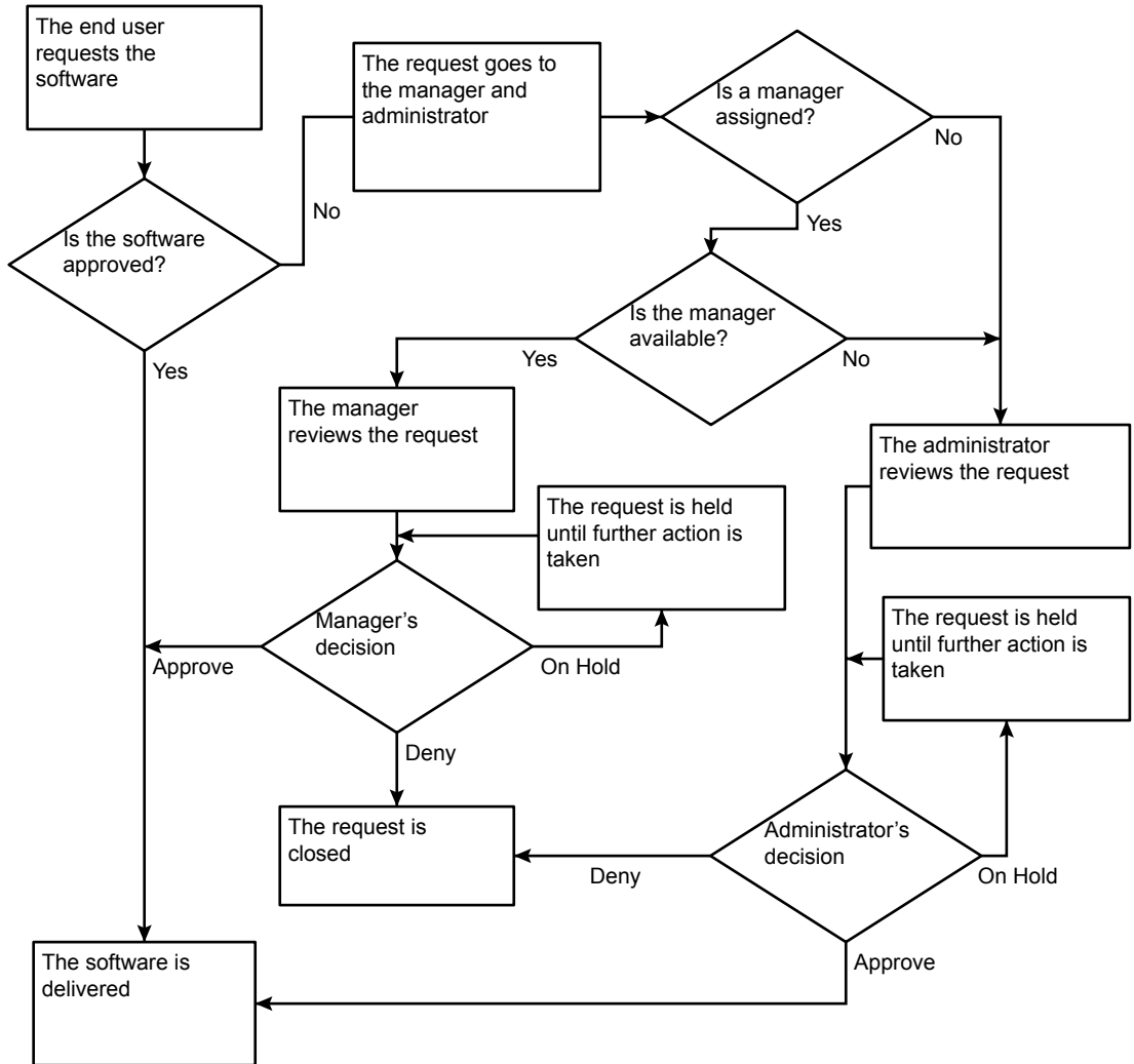
Figure 2-1 Software request work flow diagram for listed software
